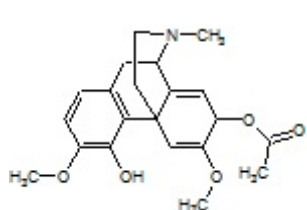
Salutaridinol-7-O-acetate
